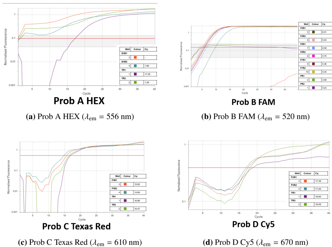
Figure 4.2. Empirical real-time qPCR amplification curves and quantification cycle ( C_q ) tables directly captured from the thermal cycler across all four optical probe channels: Probe A (HEX), Probe B (FAM), Probe C (Texas Red), and Probe D (Cy5).
