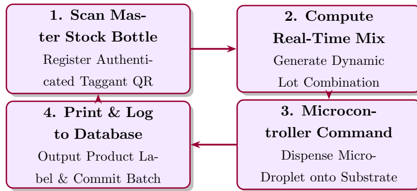
Figure 7.2: Operational workflow of the DNAx Manufacturing module governing industrial taggant registration, mixing, and dispensing.
