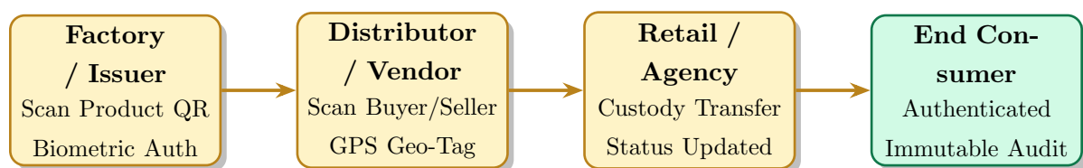
Figure 7.3: Immutable multi-party custody tracking and verification sequence governed by DNAx Vendor.
