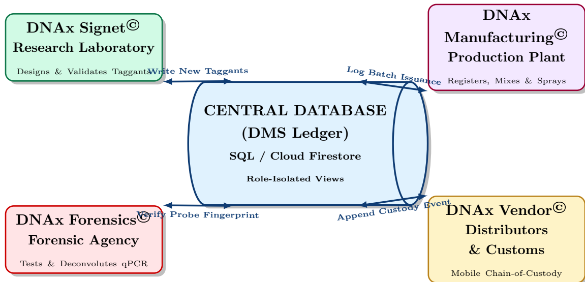
Figure 7.1: Architectural overview of the unified DNAX Digital Management System (DMS) linking all four specialized modules.
