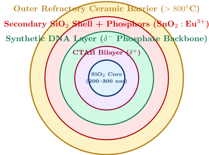
Figure 4.1: Schematic cross-section of the concentric DNA taggant composite nanoparticle showing silica core, CTAB charge-inversion layer, encapsulated DNA strands, optical phosphors, and outer ceramic barrier.
