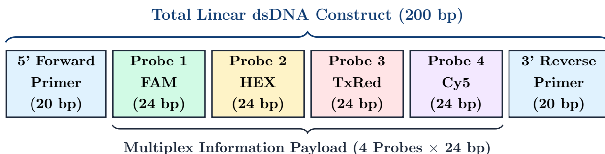
Figure 2.2: Molecular architecture of the synthesized 200 bp DNA taggant featuring flanking 20 bp primer docks and 4 internal 24 bp fluorescent probe targets.
