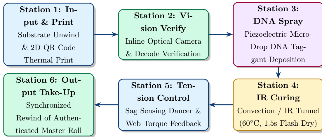
Figure 5.3: Schematic block diagram of the automated 6-station roll-to-roll DNA taggant spray and curing assembly line.
