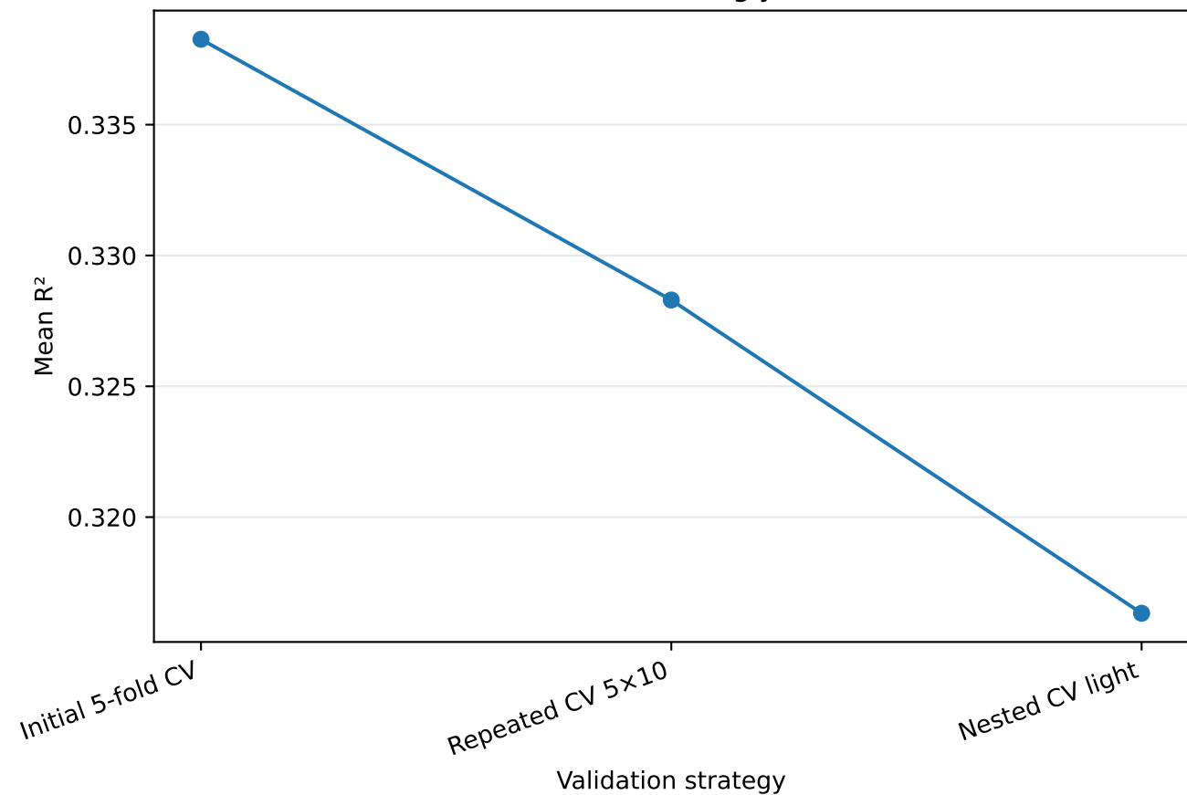
Performance under increasingly robust validation
