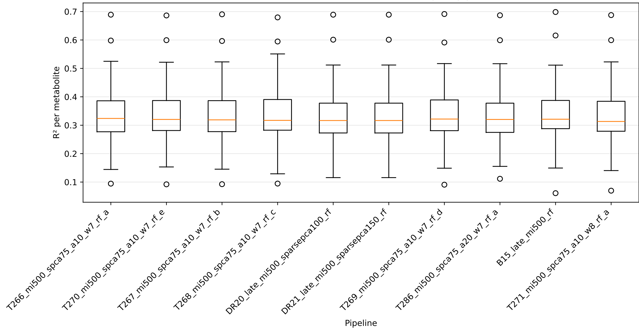
Distribution of R^2 across metabolites for top 10 pipelines
