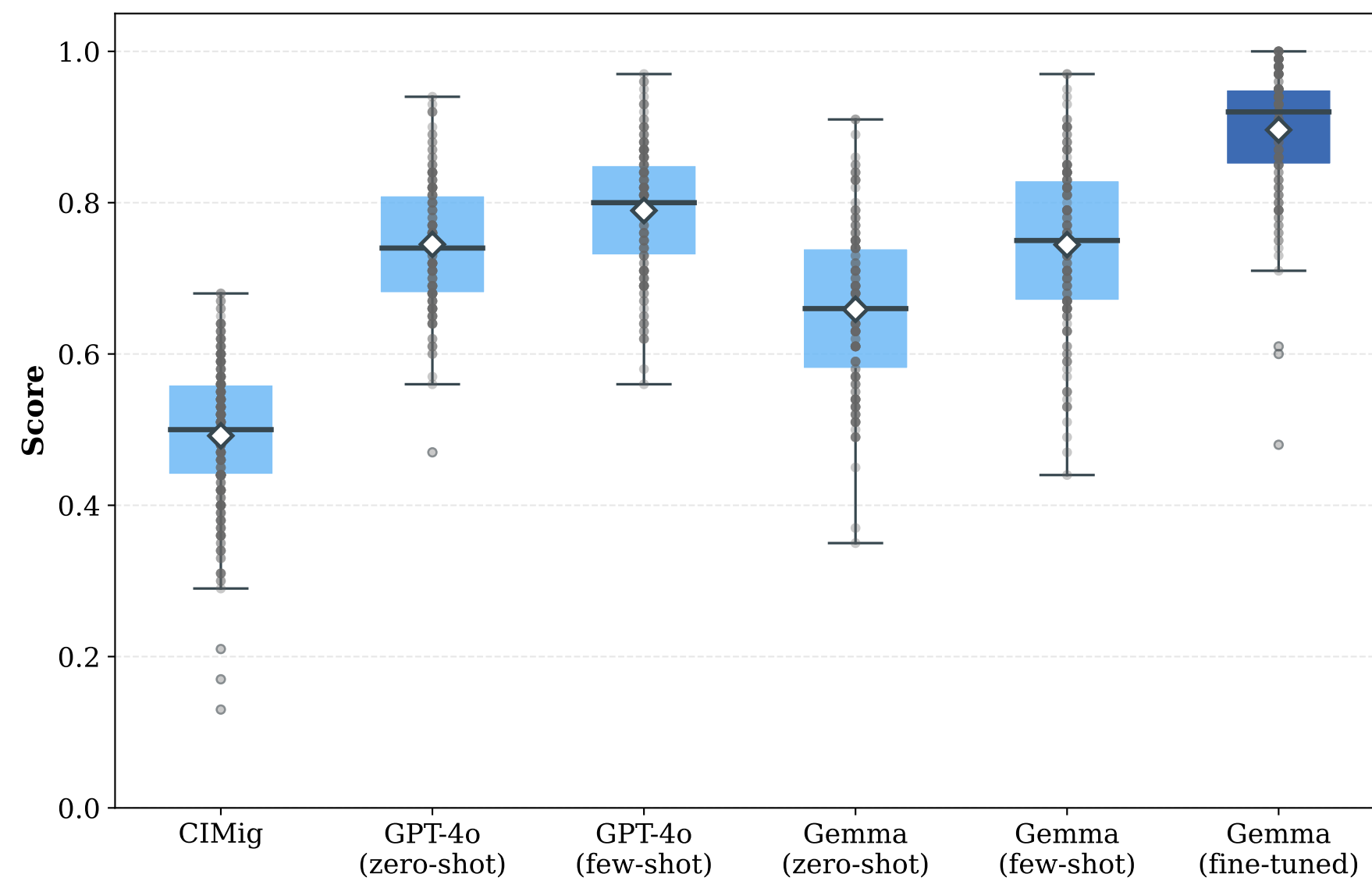
Cosine Similarity
