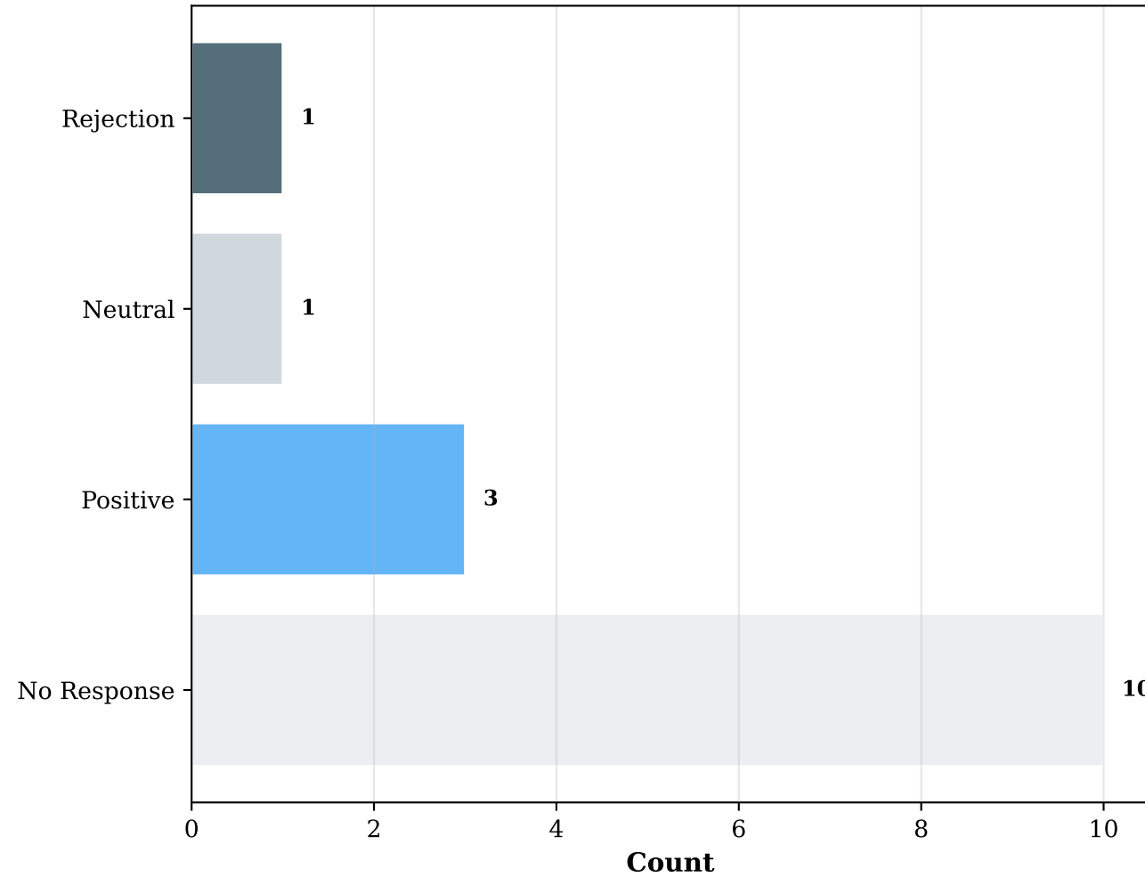
Travis → GHA
