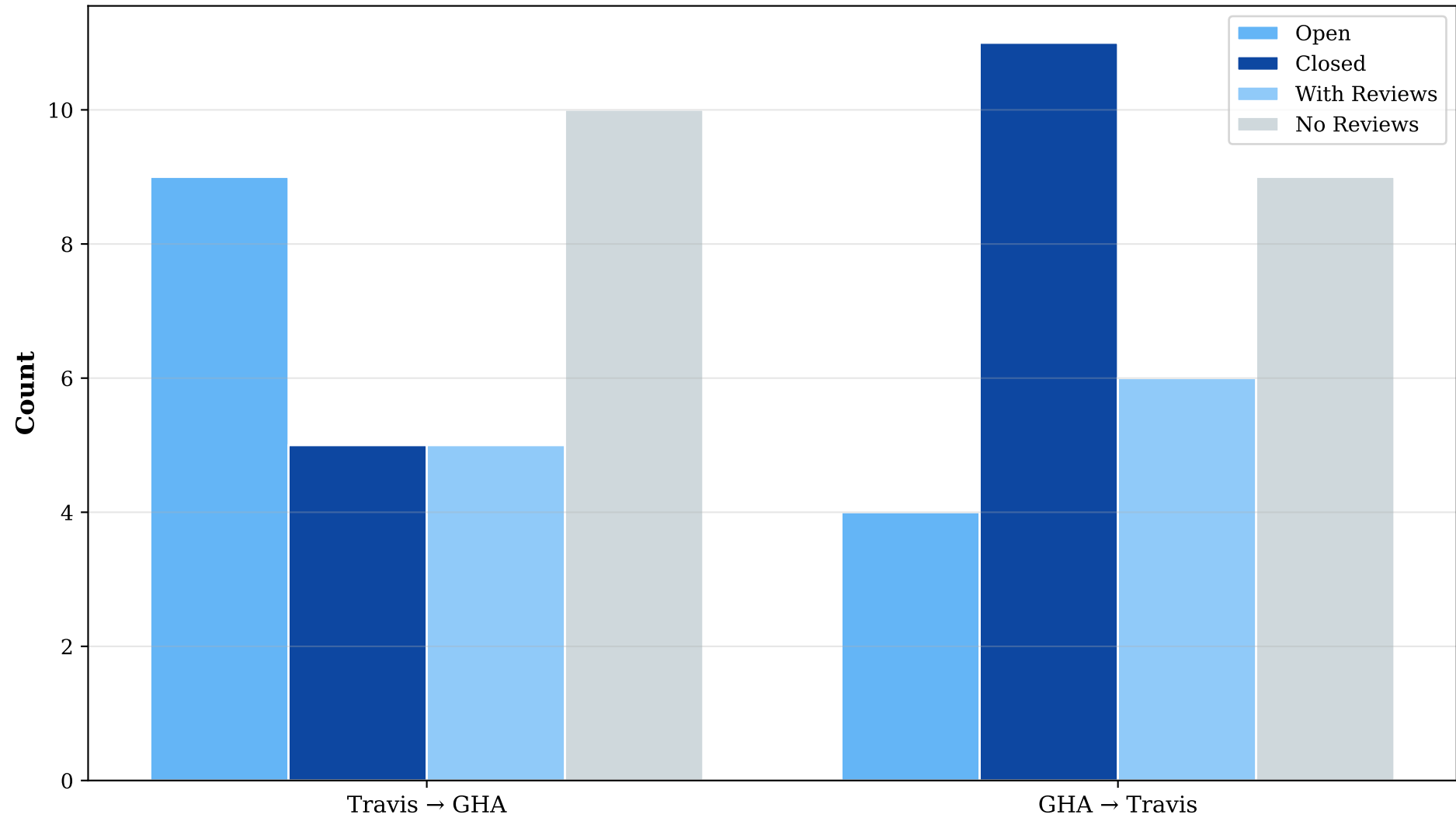
Pull Request Status Distribution
