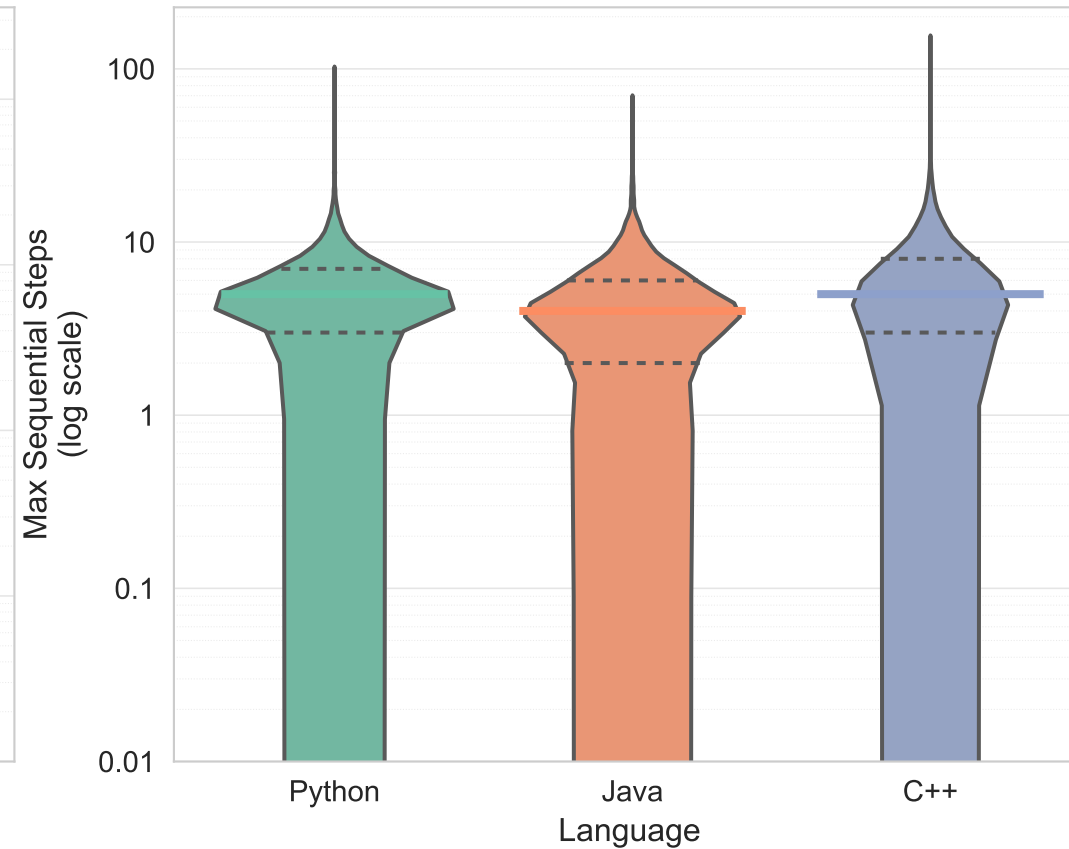
Max Sequential Steps
