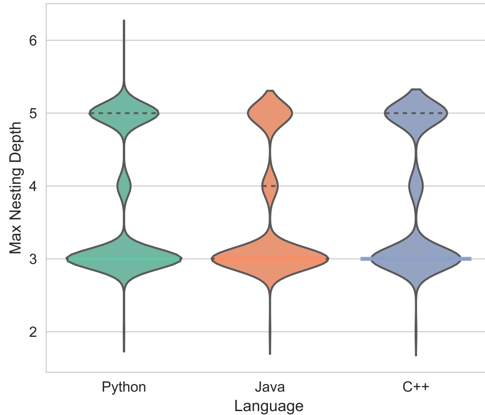
Max Nesting Depth
