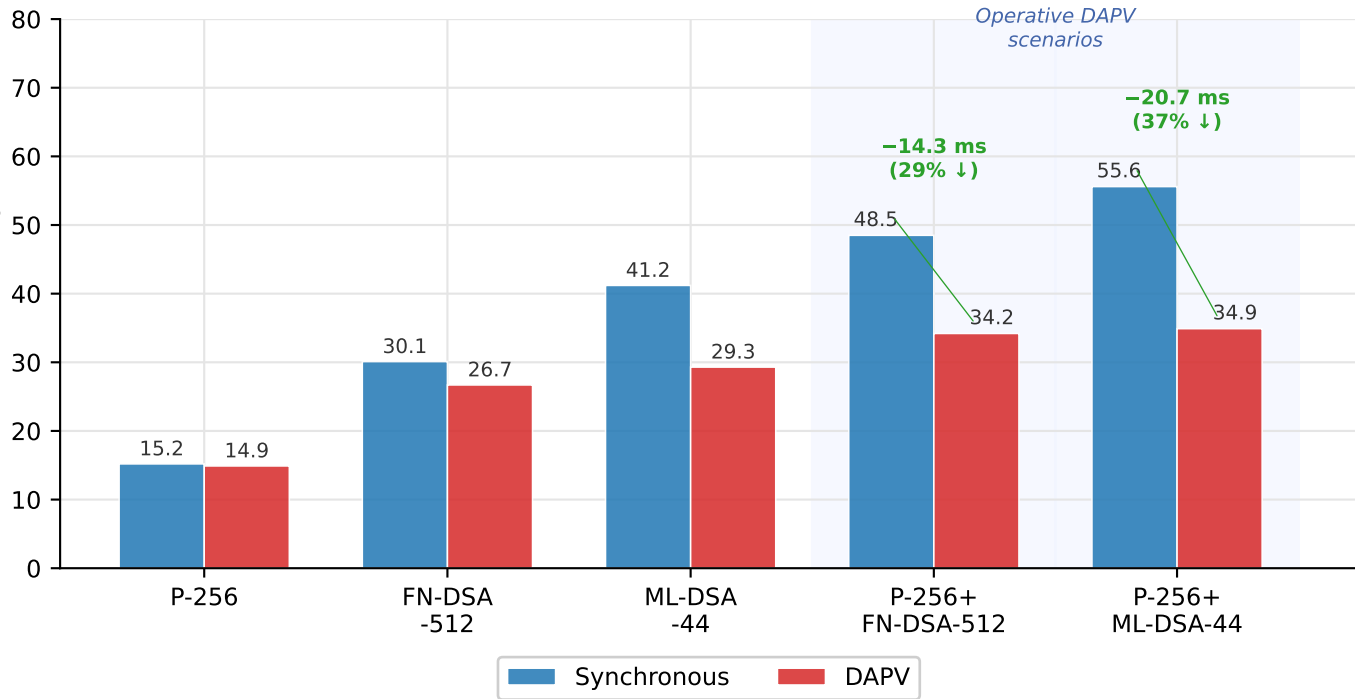
Handshake latency (ms)
