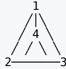
K_4 (planar drawing)
