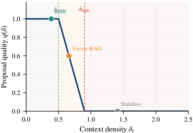
Context-rot degradation model (Eq.~1)
