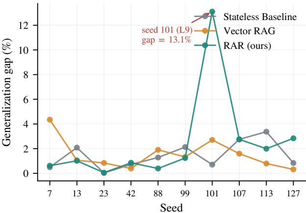
Per-seed generalization gap on digits
