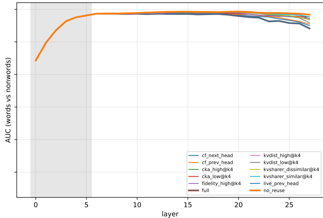
Qwen2.5-1.5B: retrained readout
