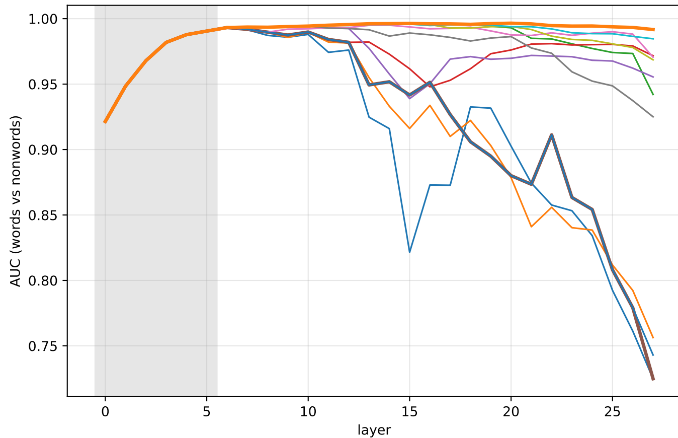
Qwen2.5-1.5B: frozen readout
