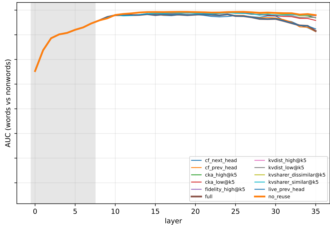
Qwen2.5-3B: retrained readout
