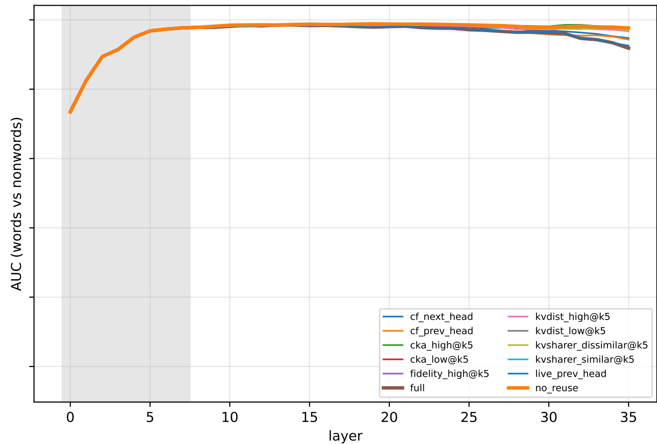
Qwen3-4B-Base: retrained readout
