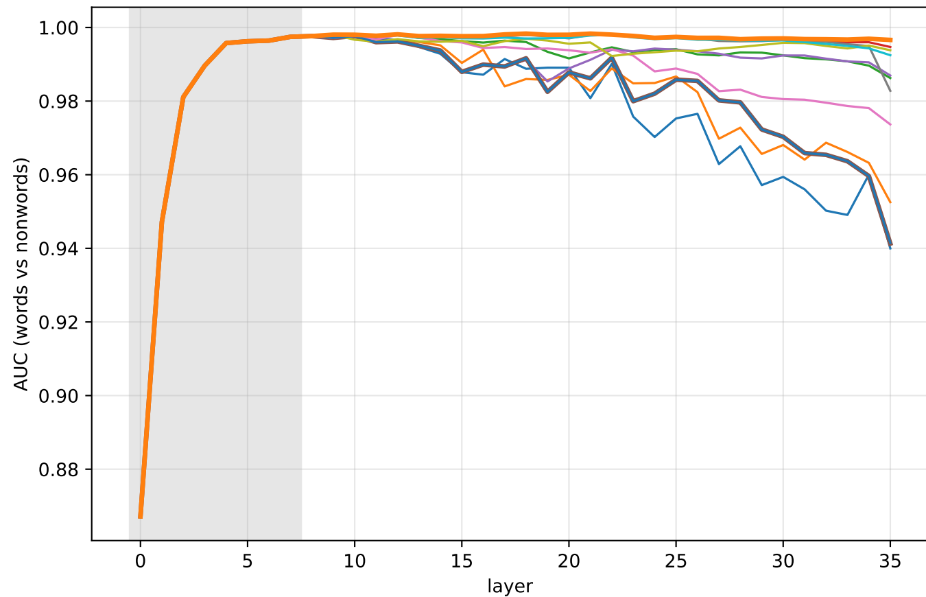
SmolLM3-3B-Base: frozen readout
