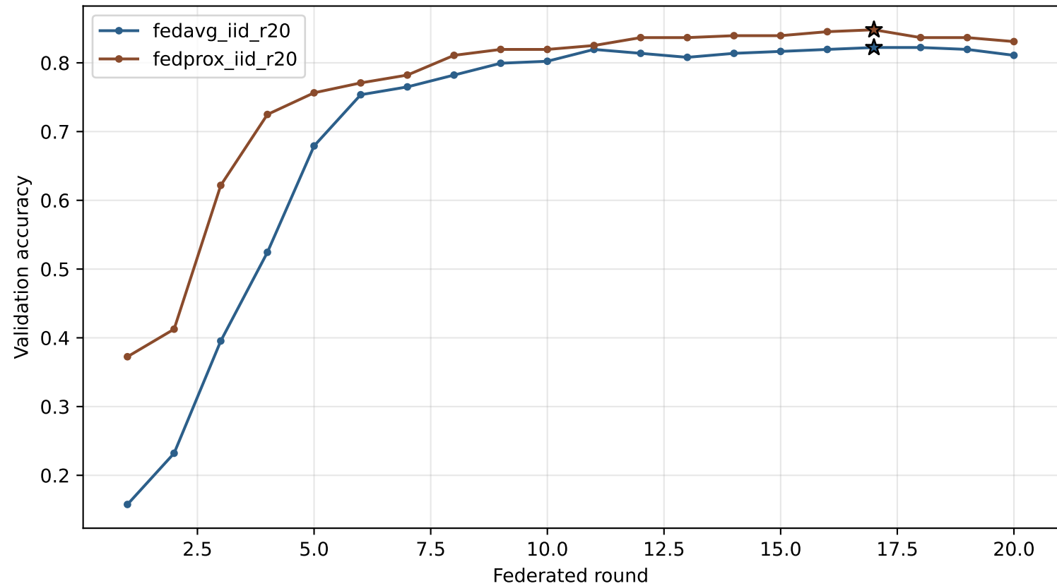
Validation learning curves (star = best-val round)
