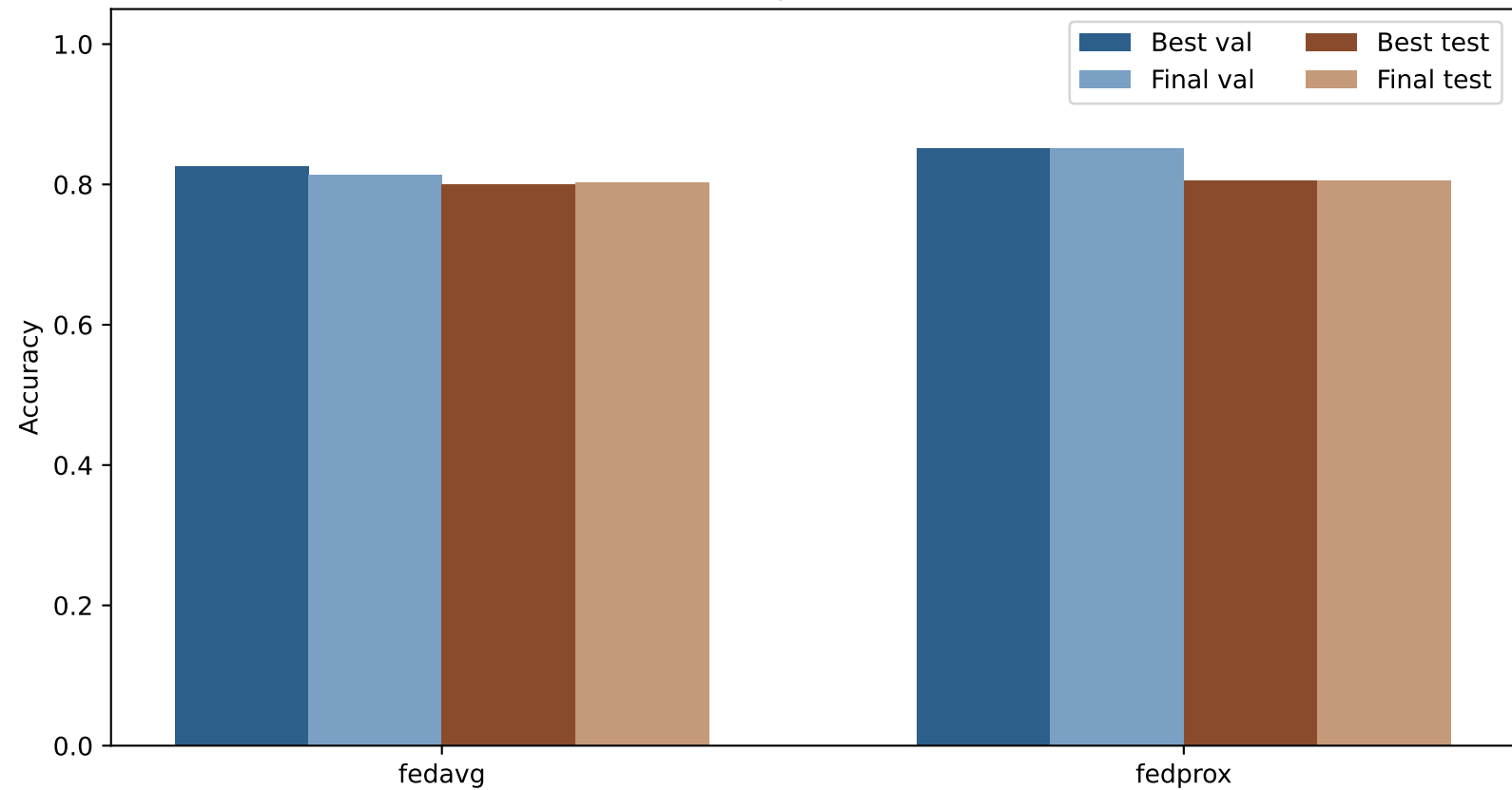
Best-val checkpoint vs final round
