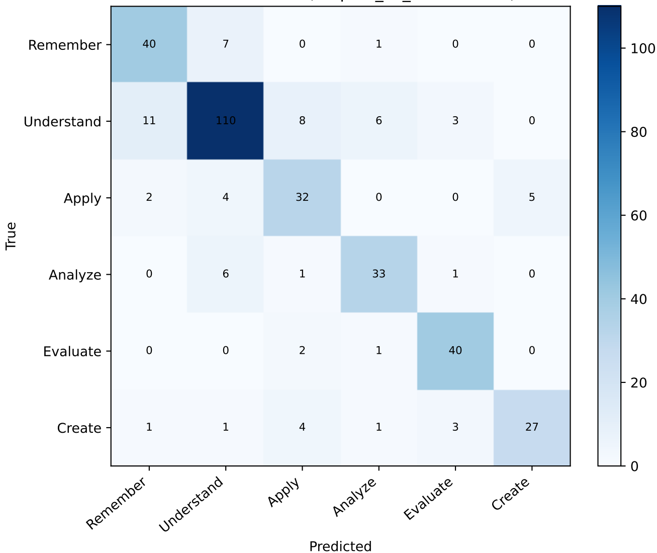
Confusion matrix (fedprox_iid_r20 best r20)
