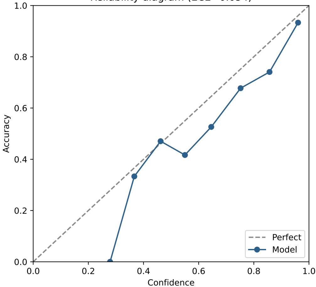
Reliability diagram (ECE=0.054)
