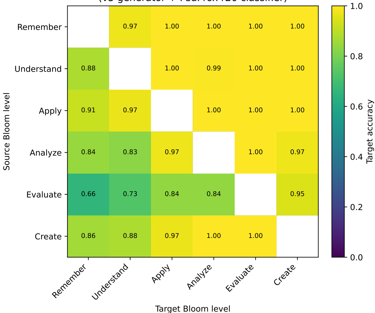
Source→target Bloom target accuracy (v3 generator + FedProx r20 classifier)
