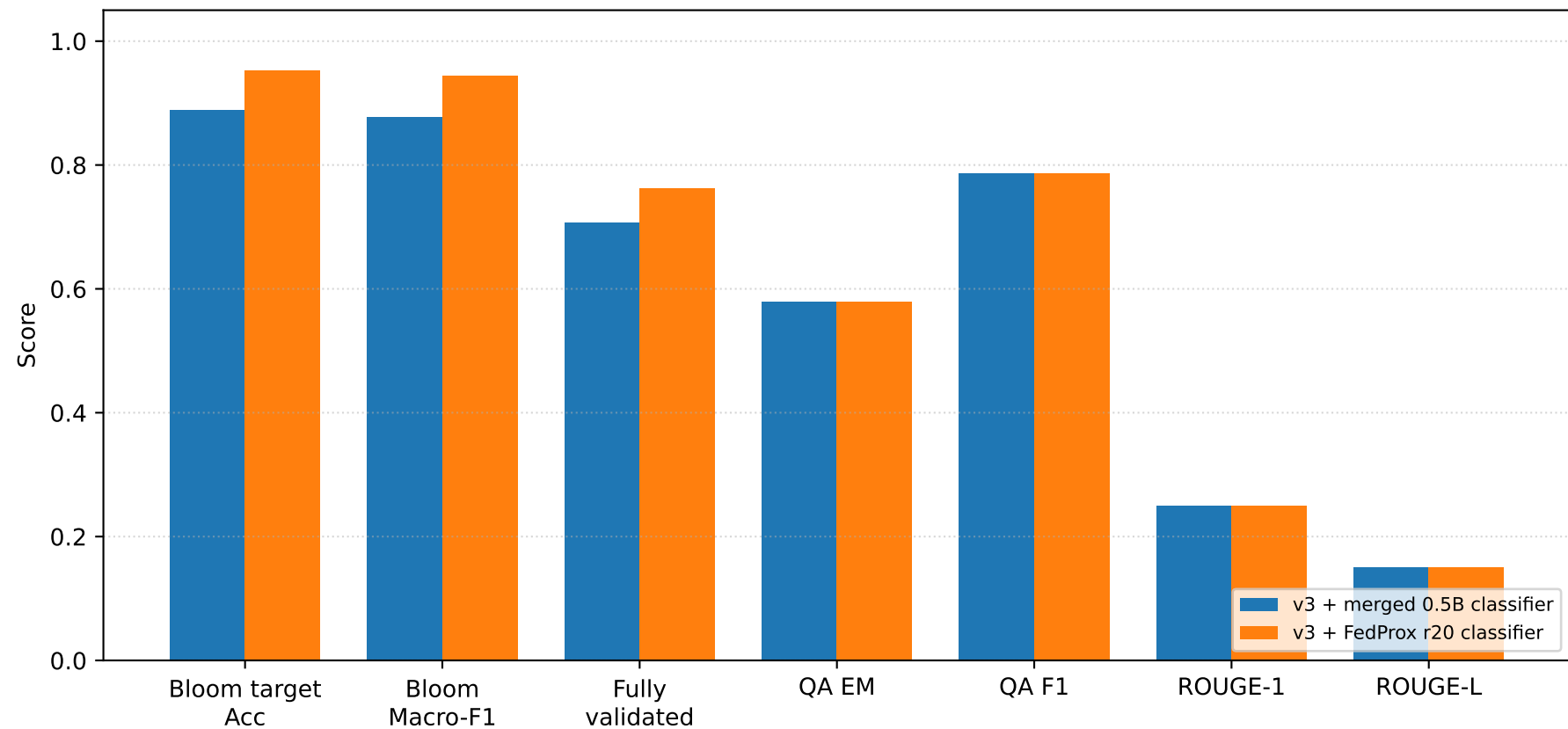
Multitask v3 test metrics (frozen test; N=8321)
