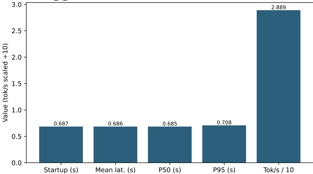
Q4_K_M GGUF micro-benchmark (size=986.0 MB, RSS=1300 MB)
