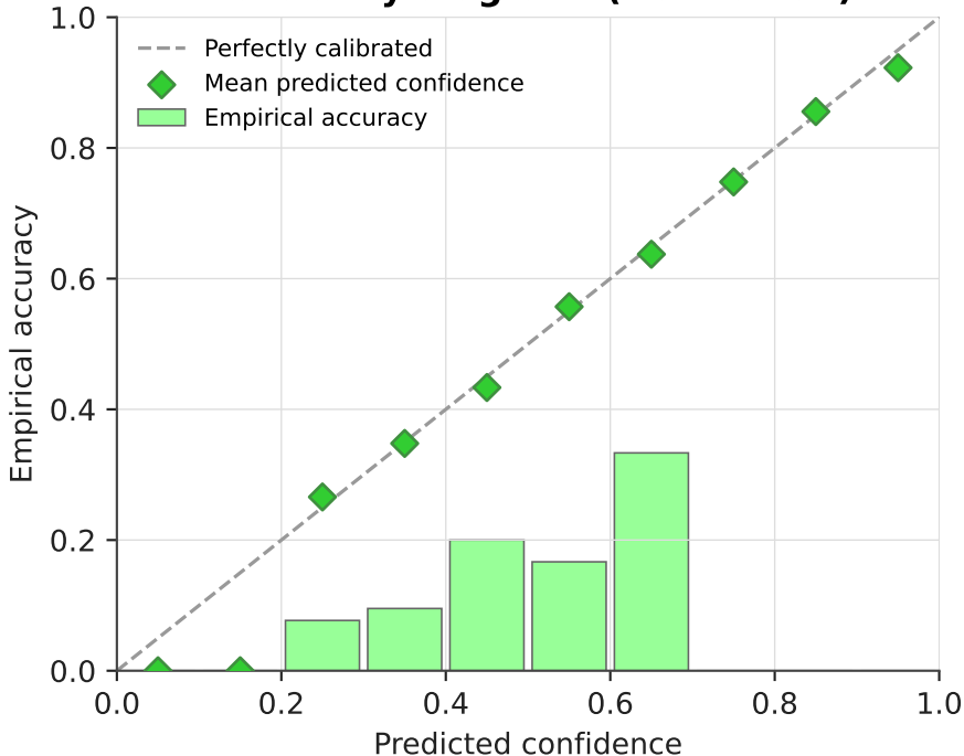
Reliability diagram (ECE=0.292)
