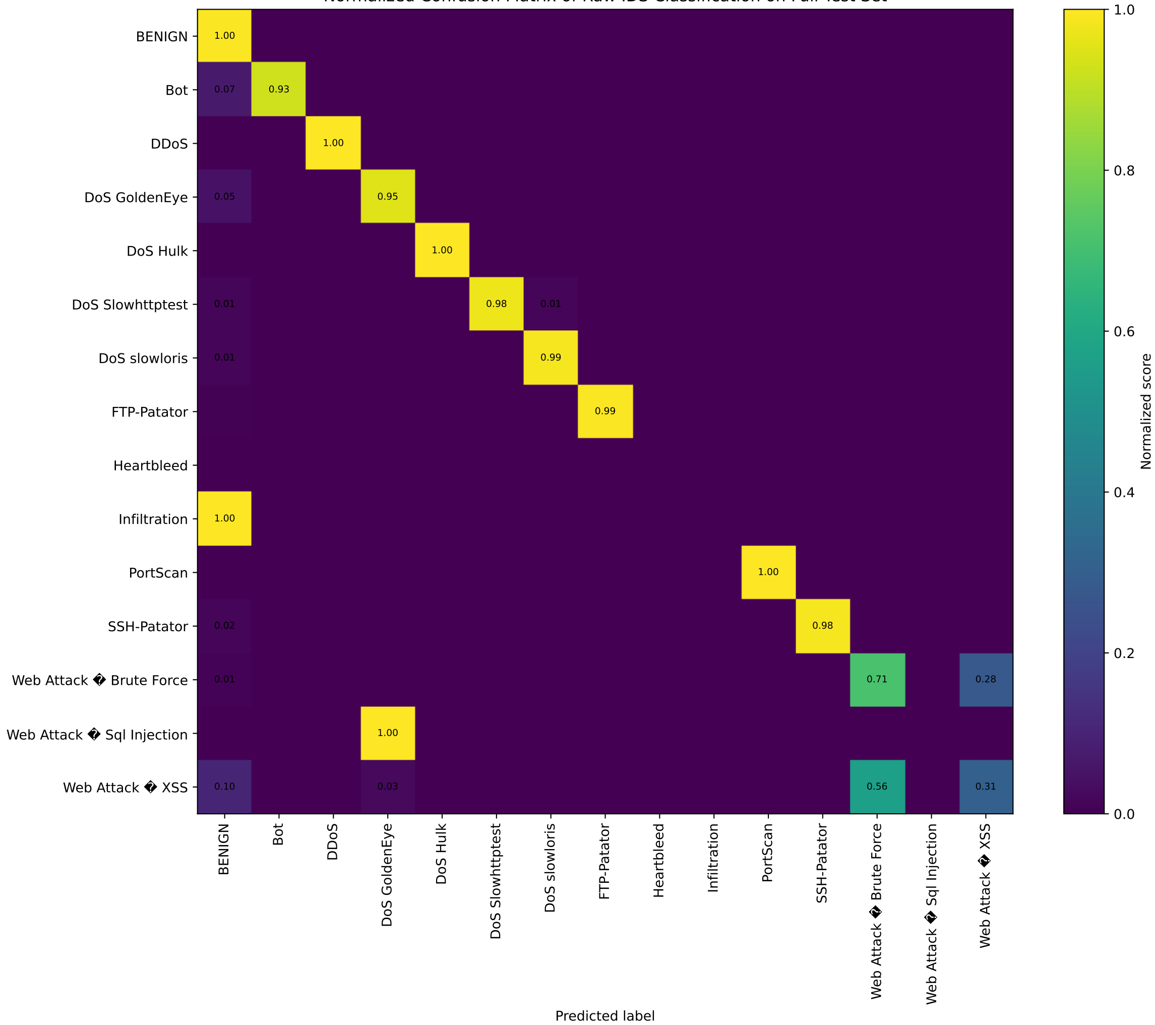
Normalized Confusion Matrix of Raw IDS Classification on Full Test Set
