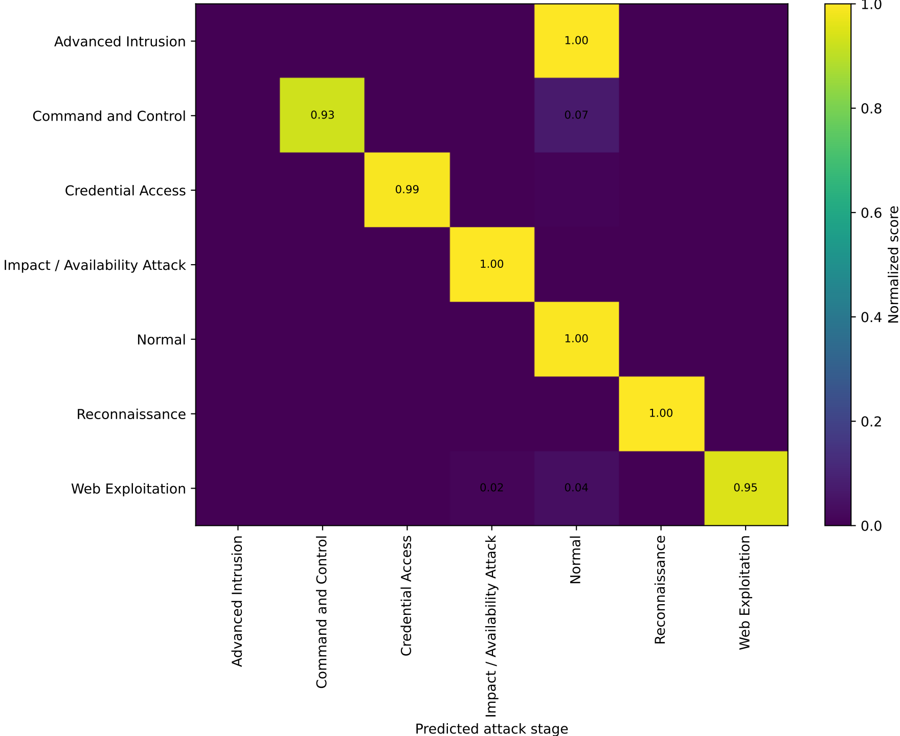
Normalized Confusion Matrix of Attack-Stage Classification on Full Test Set
