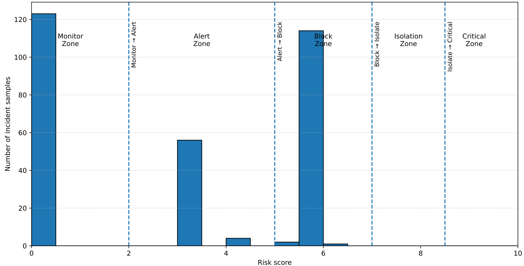
Risk Score Distribution Across Response Policy Zones
