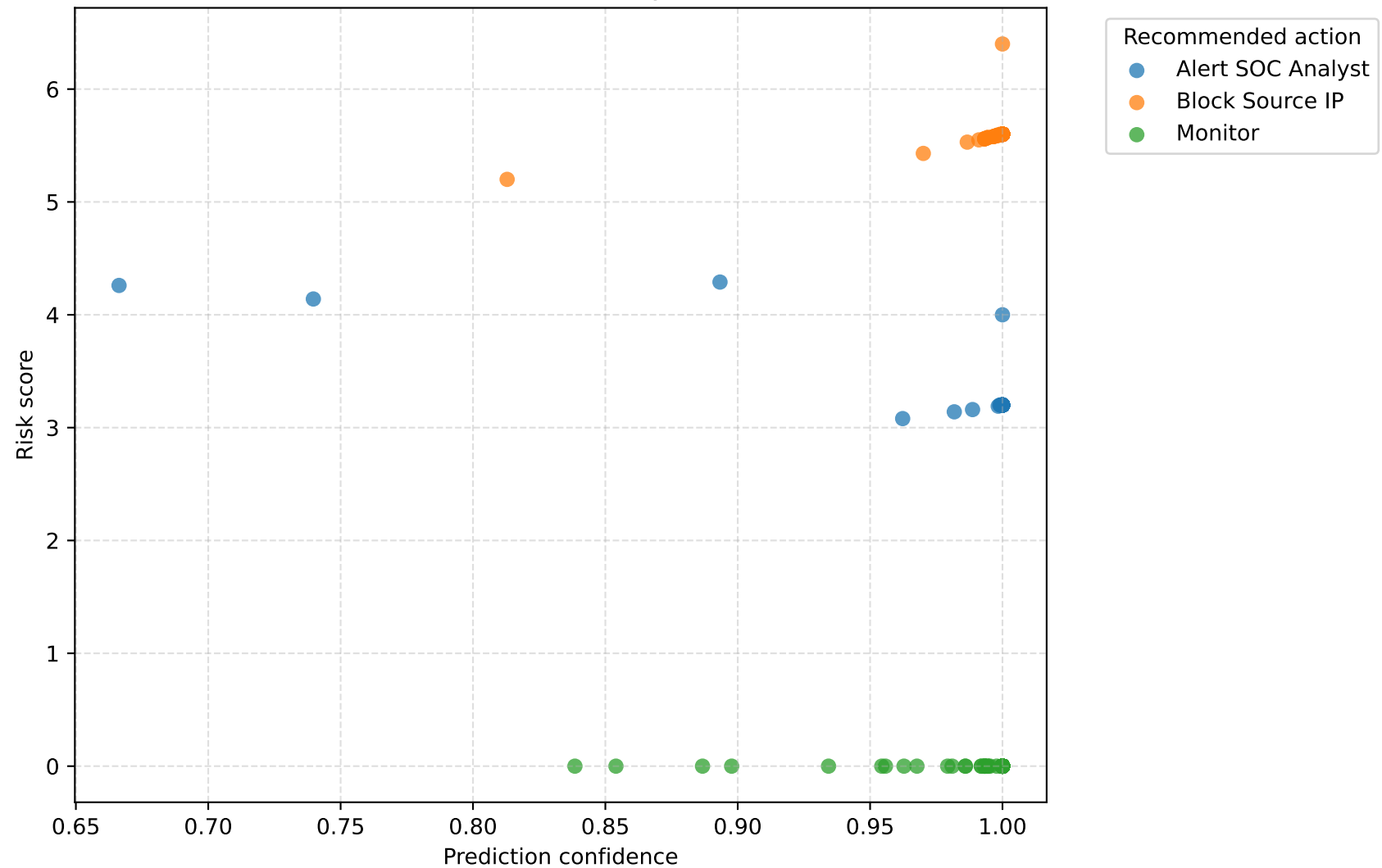
Prediction Confidence vs Risk Score by Recommended Action
