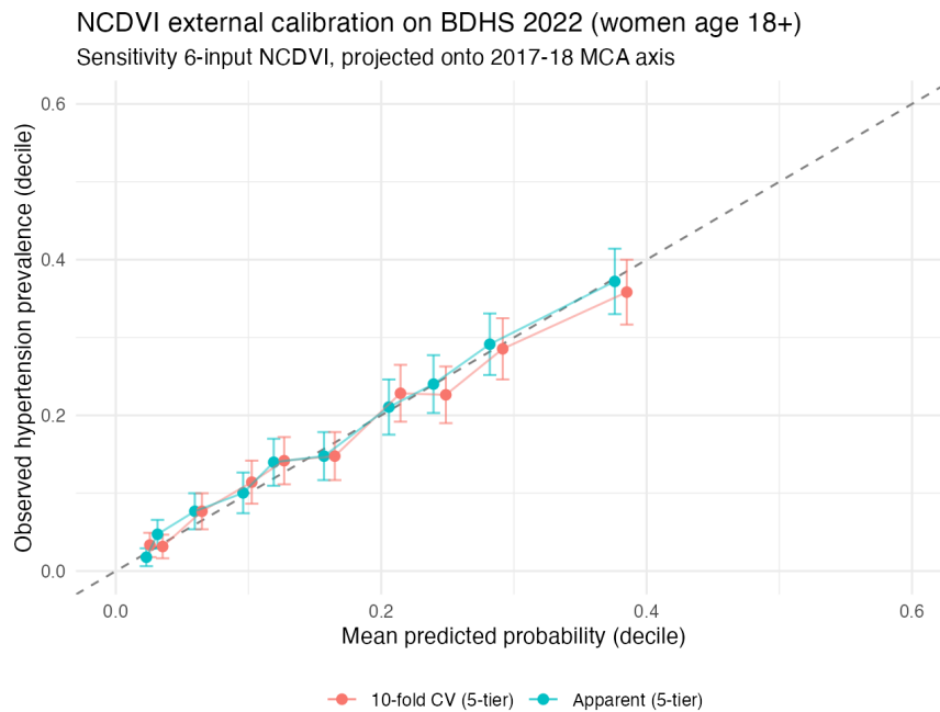
Figure 3: External calibration of the six-input sensitivity NCDVI on the BDHS 2022 women's biomarker subsample (N = 5,080). Points show mean predicted probability against observed hypertension prevalence within deciles of predicted risk, for both the apparent and tenfold cross-validated predictions. Dashed line indicates perfect calibration.
