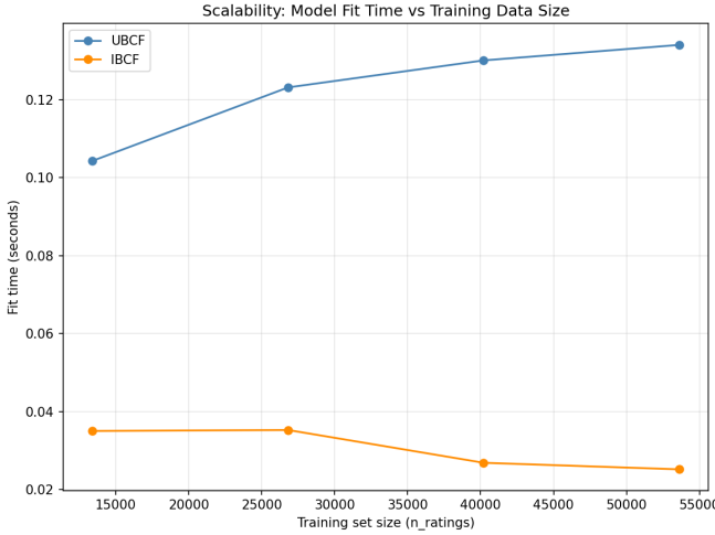
Fig. 4. Model fit time as a function of training set size.
