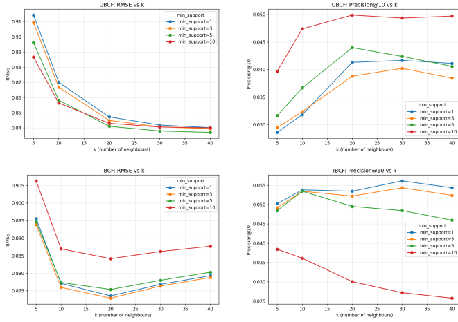
Fig. 2. RMSE and Precision@10 as a function of neighborhood size k , for each \text{min\_support} value tested. Top row: UBCF. Bottom row: IBCF.
