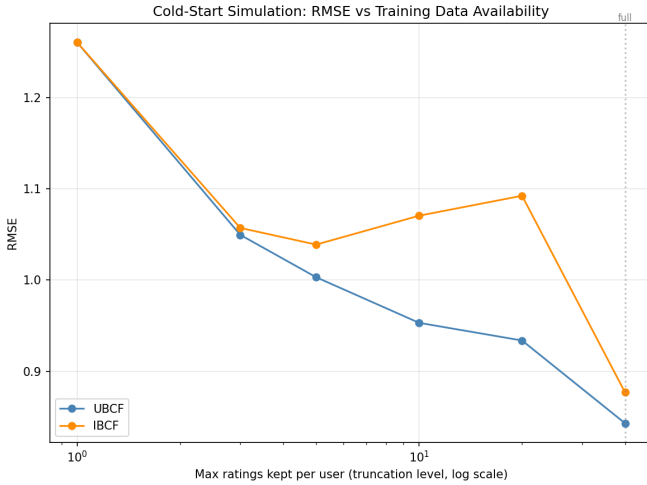
Fig. 3. RMSE vs. training data availability (simulated cold-start).
