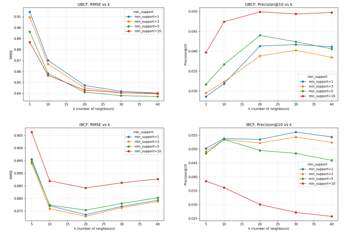
Fig. 2. RMSE and Precision@10 as a function of neighborhood size k , for each min_support value tested. Top row: UBCF. Bottom row: IBCF.
