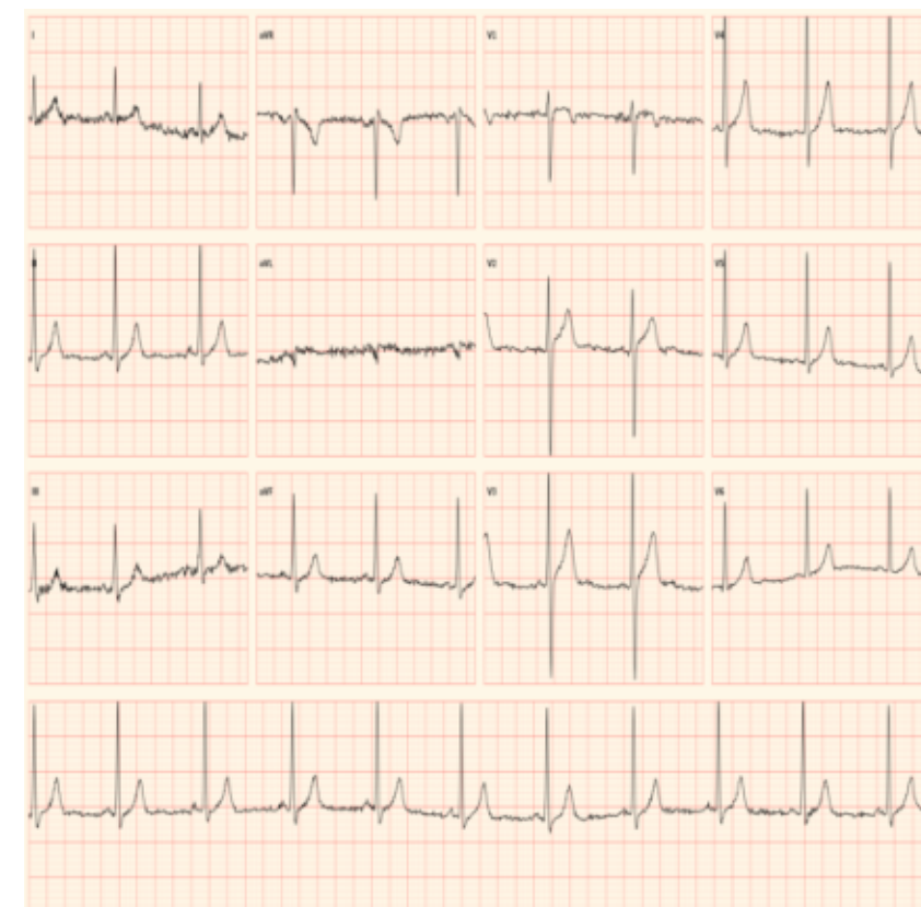
Grad-CAM
