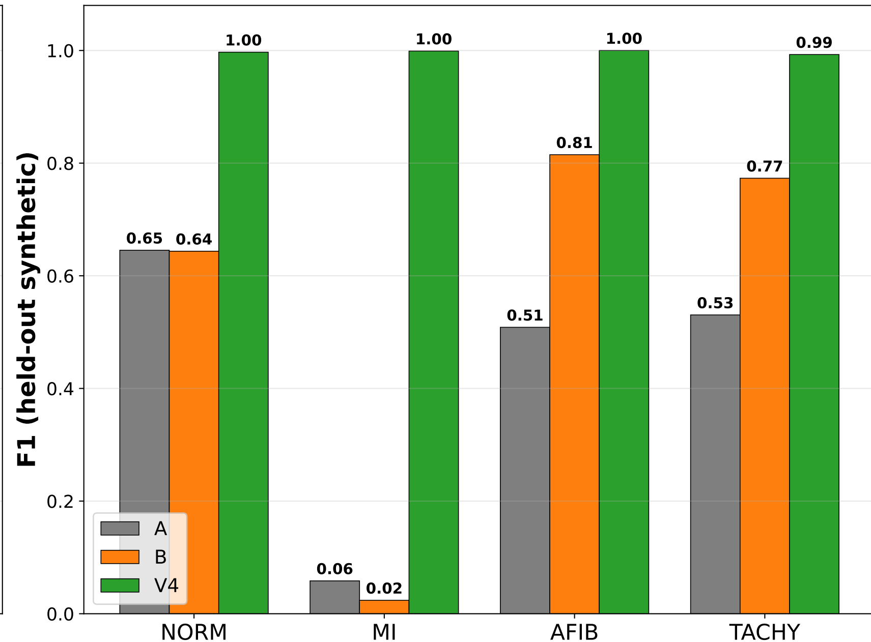
Per-class F1 on held-out synthetic (real-only & diffusion-only collapse on MI)
