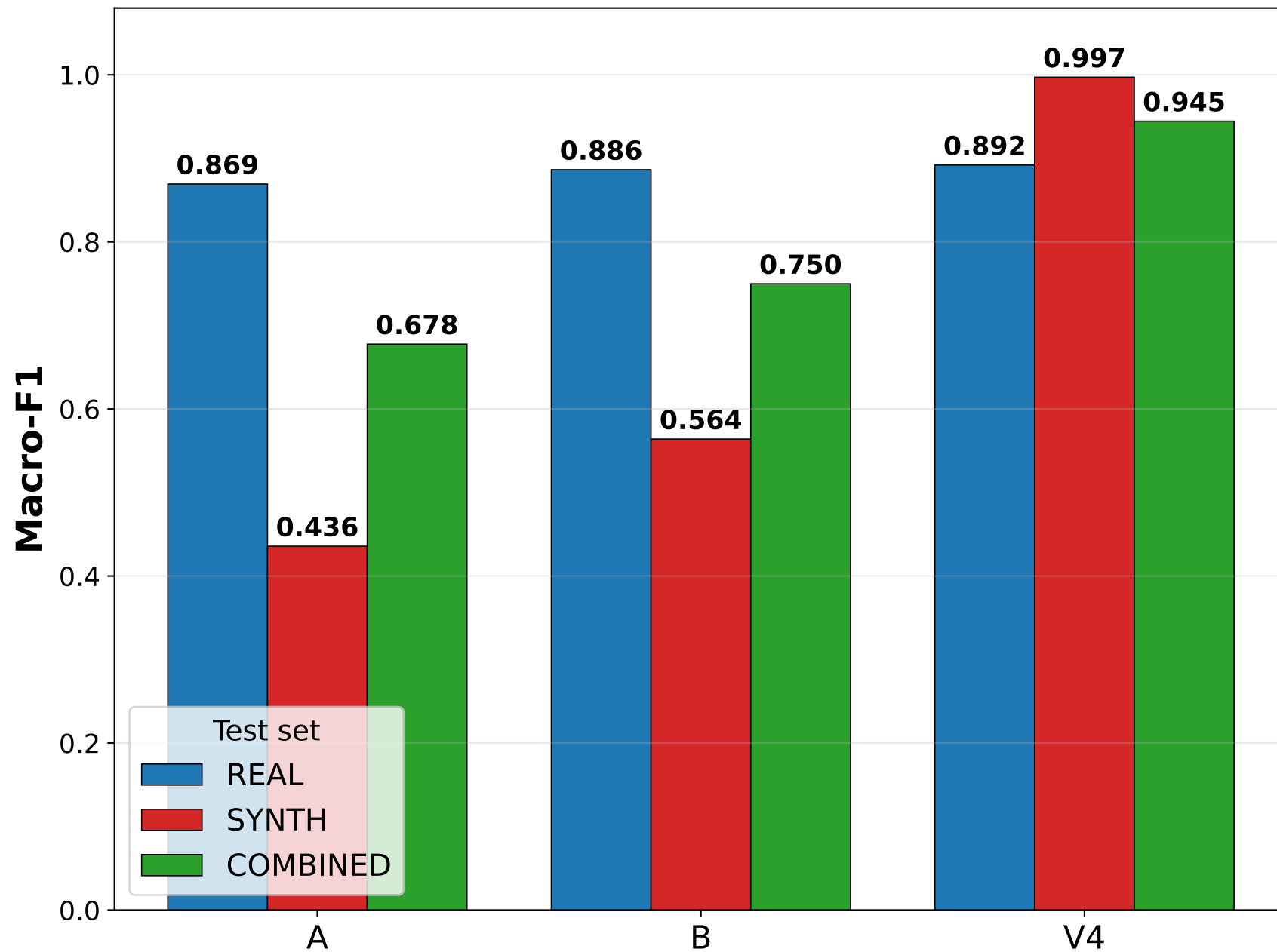
Macro-F1: Real vs Held-out Synthetic vs Combined (50:50)
