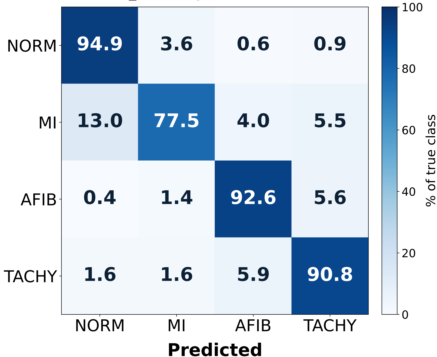
A_realonly — REAL test
