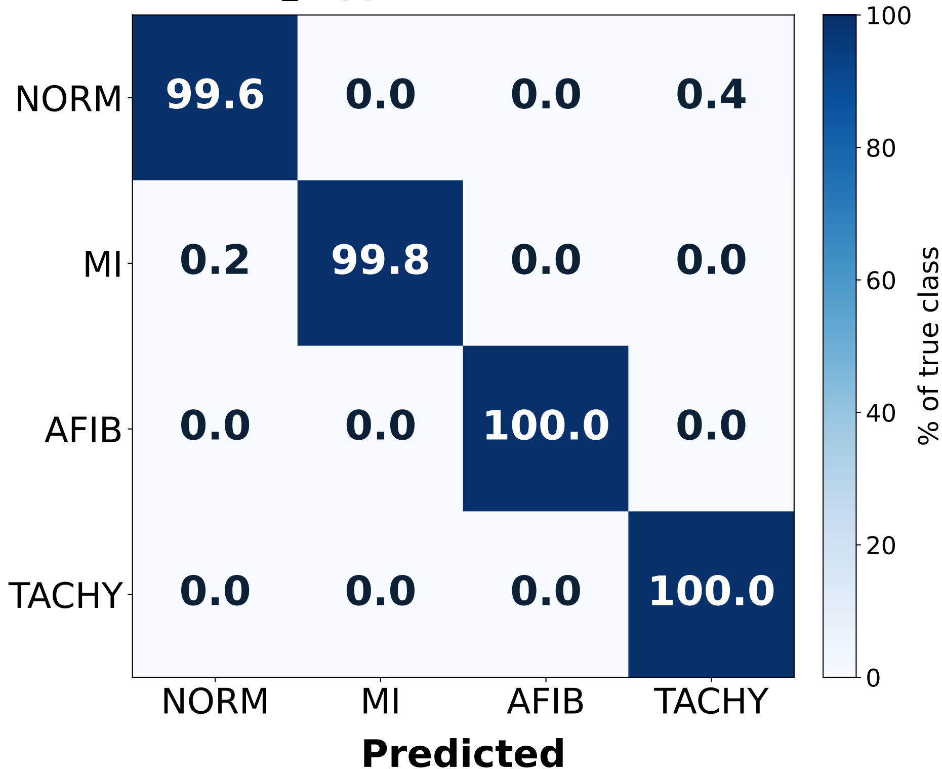
V4_capped — SYNTH test
