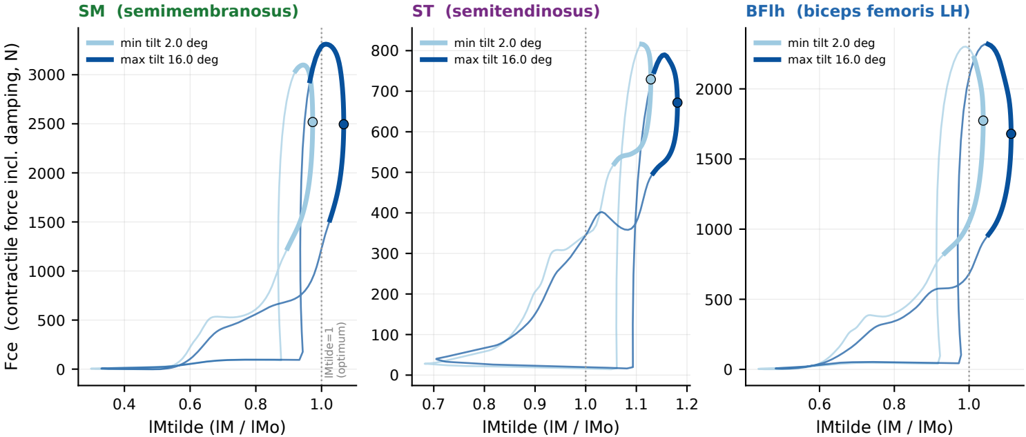
Figure S1 | Force-length operating region (biarticular hamstrings, min vs max tilt, N=100)
