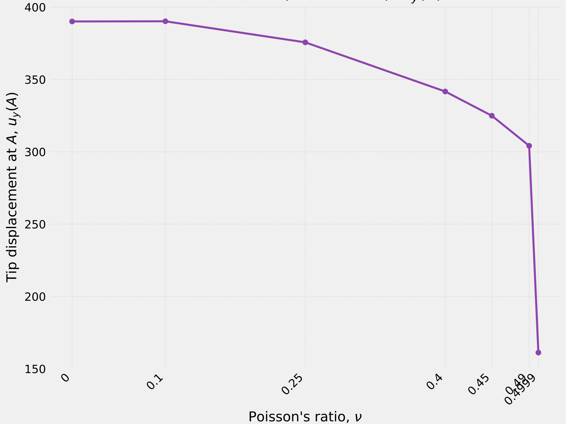
Cook's membrane (finest mesh): u_y(A) vs \nu
