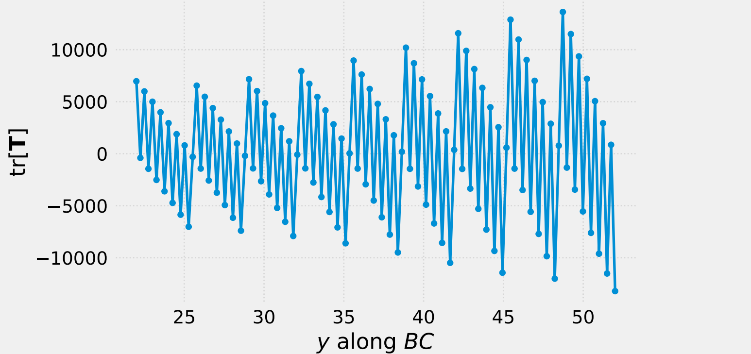
Cook's Problem: \text{tr}[\mathbf{T}] along BC (near-edge element eval, averaged)
