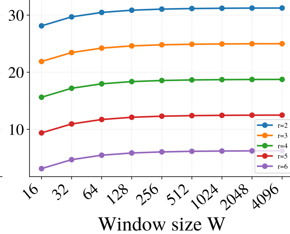
Qwen2.5-7B
