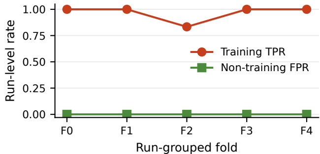
Aggregate: 22/23 TP, 0/95 FP
