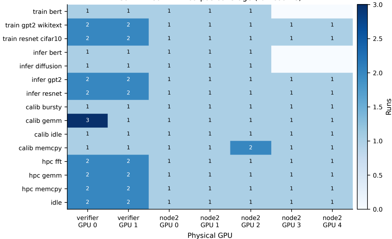
Committed NVML corpus coverage (run counts)
