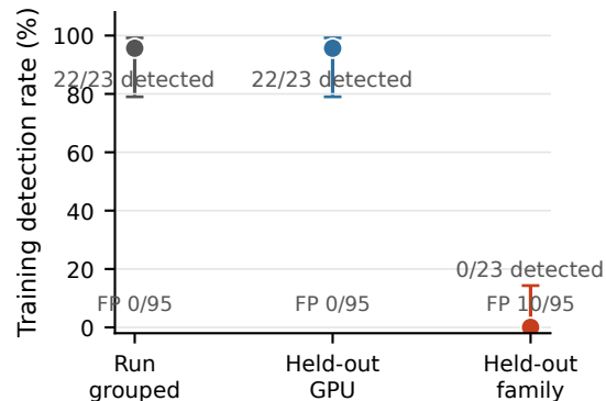
(b) NVML fails on unseen families
