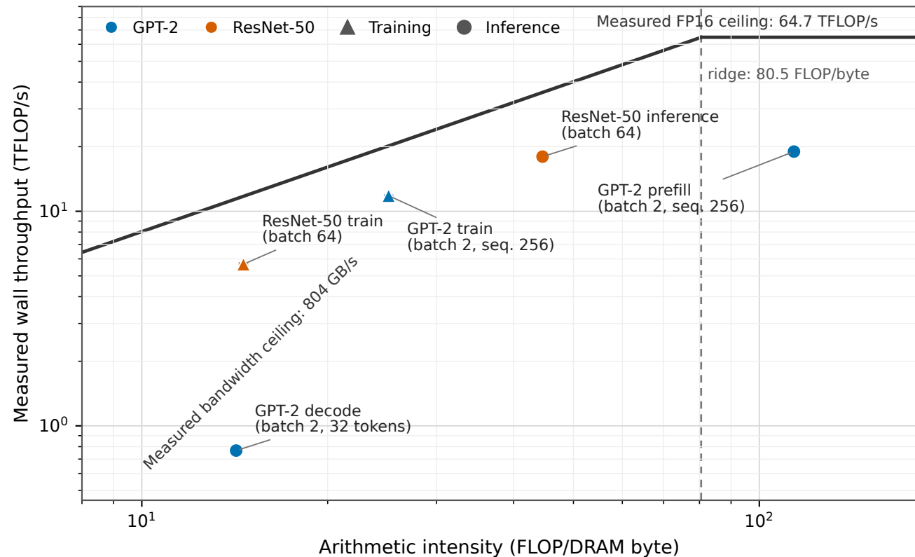
RTX 3090 application roofline (FP16, 200 W) Matched training and inference; median of 3 runs, whiskers show range
