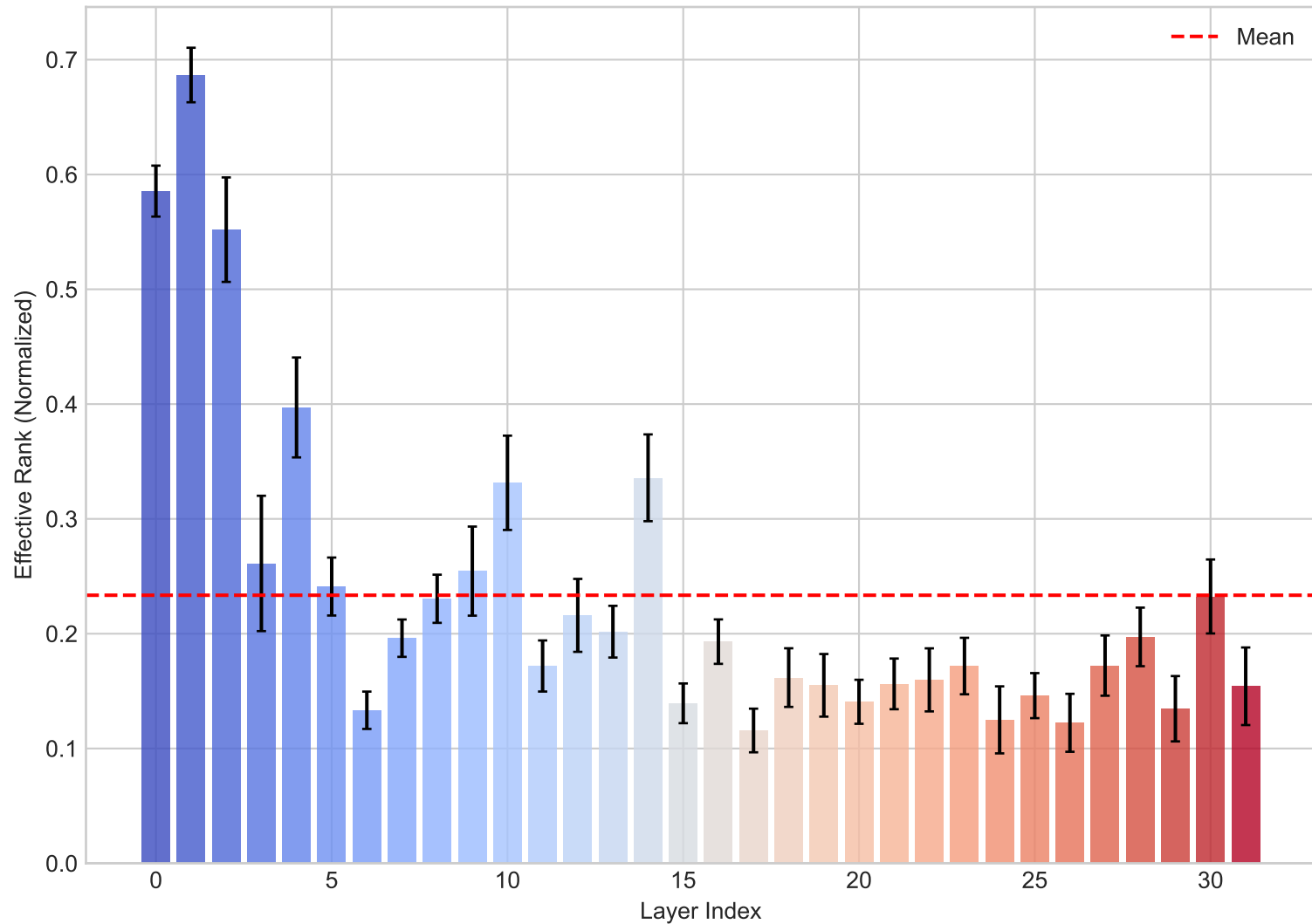
Effective Rank per Layer (Detailed)
