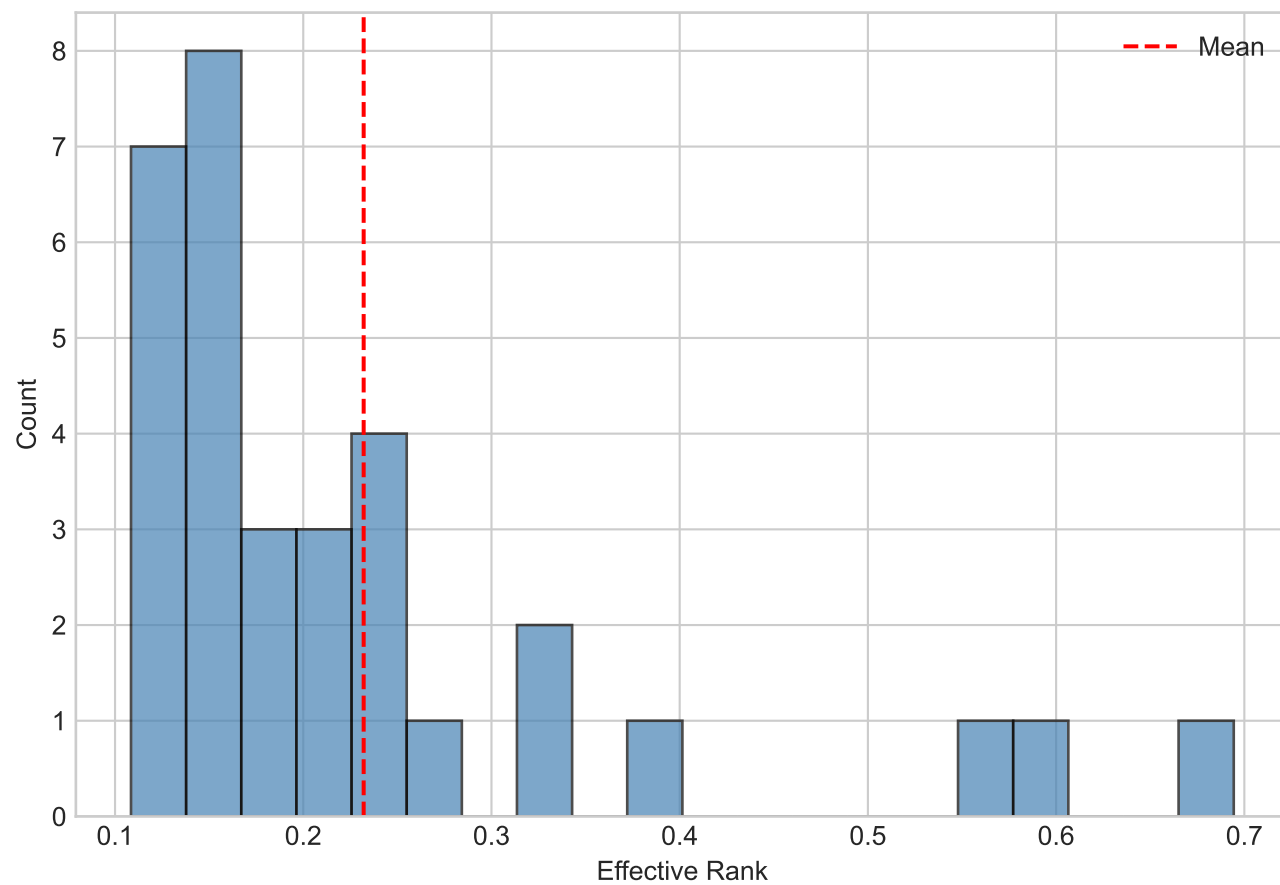
Distribution of Effective Ranks
