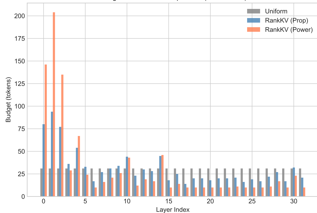
Budget Allocation Comparison (Total=1000)
