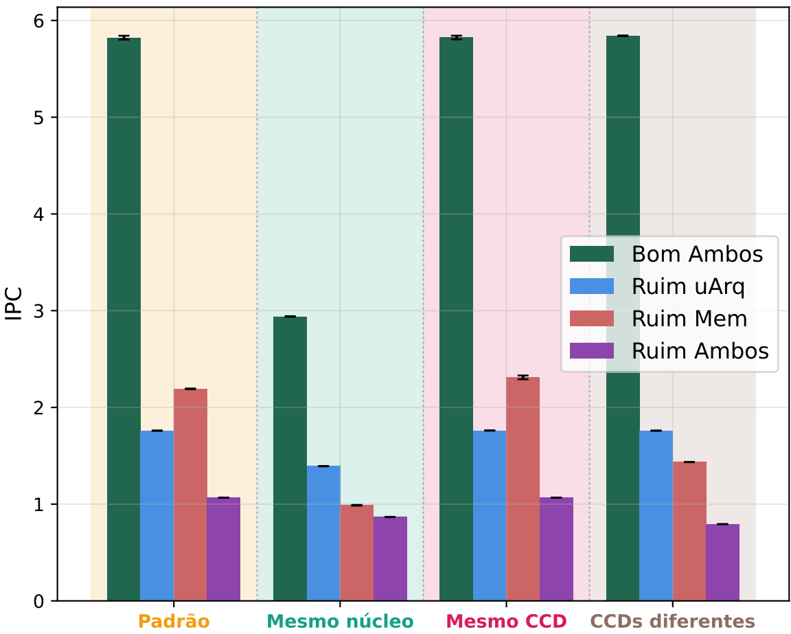
IPC (Instr/Ciclo) (2 Threads)
