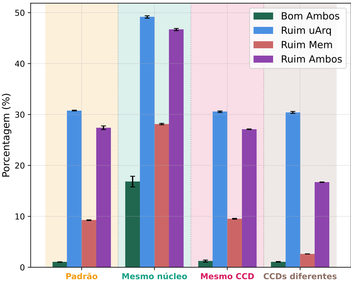
Starvation de Frontend (% de Ciclos) (2 Threads)
