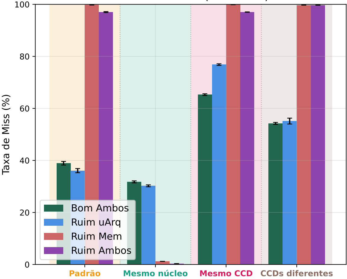
Taxa de Miss L1 (2 Threads)
