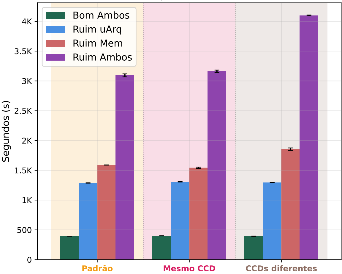
Tempo (3 Threads)
