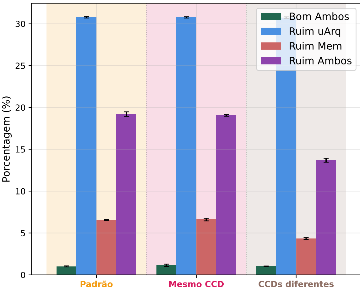
Starvation de Frontend (% de Ciclos) (3 Threads)
