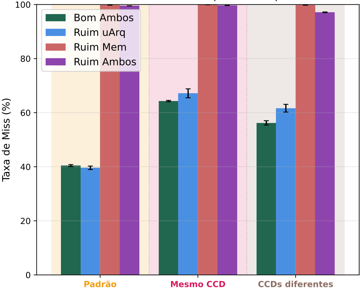
Taxa de Miss L1 (3 Threads)
