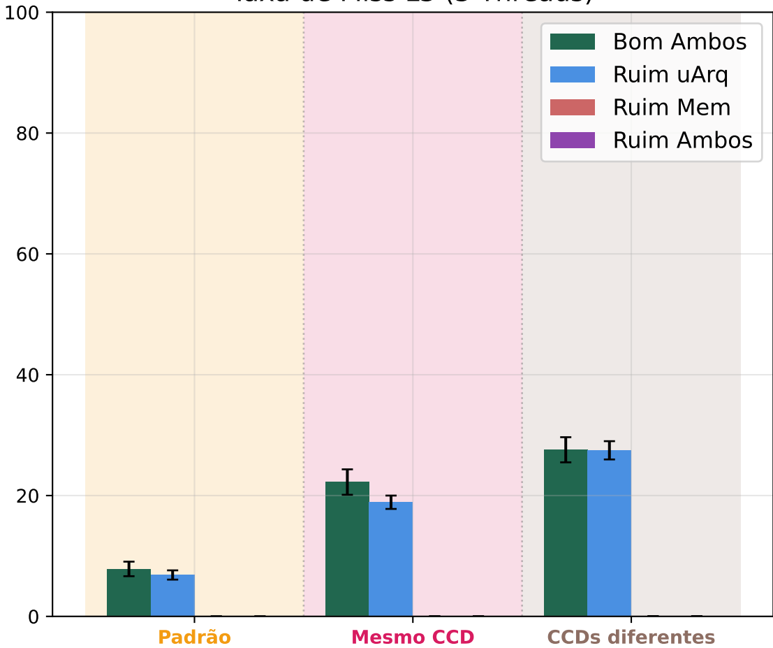
Taxa de Miss L3 (3 Threads)
